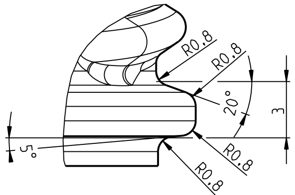
Detail Ring 5:1
